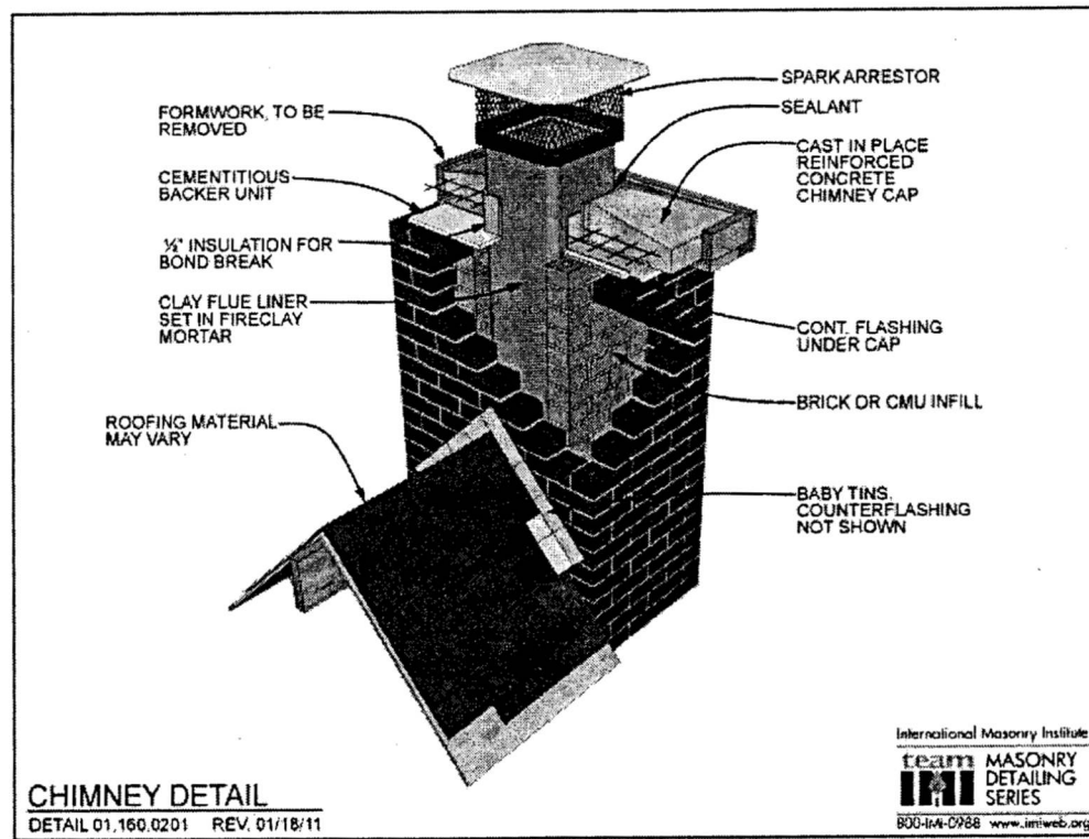
Gable End Chimney
